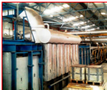
FCPTUNNEL KILN
